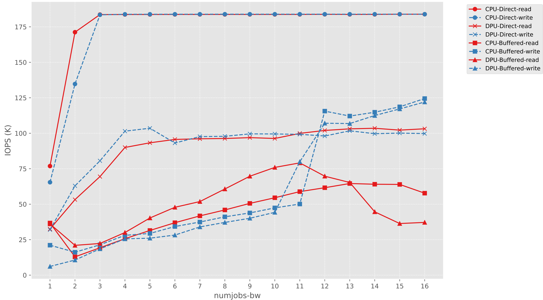
IOPS vs numjobs-bw (CPU vs DPU, Direct vs Buffered)
